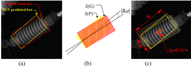
Fig. 5. Candidate bounding box generation. (a) Ground-truth bounding box and the bounding box predicted by the BLN. (b) Overlap and angle differences. (c) Seed region and candidate bounding boxes.
