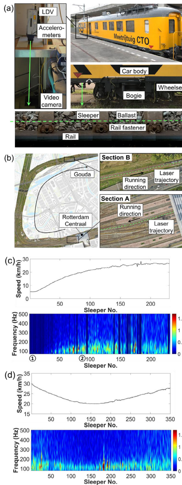
FIGURE 9 Field measurements. (a) CTO train instrumented with a laser Doppler vibrometer (LDV); (b) train route and two selected sections (aerial photographs used from GeoInformatie Portaal of ProRail https://maps.prorail.nl/ ); (c) train speed and spectrum of imputed signal for each sleeper in Section A; (d) train speed and spectrum of imputed signal for each sleeper in Section B.
