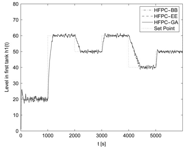
Fig. 12. Simulation test. Controlled-variable response.
