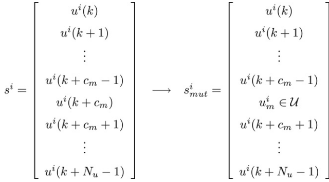
Fig. 3. Mutation of an individual in c_m th place.
